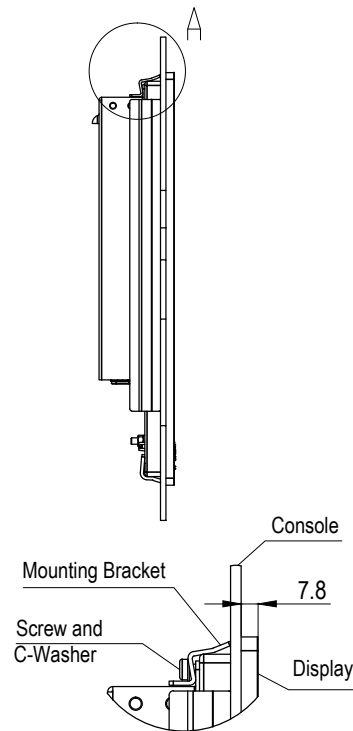
DETAIL A SCALE 1 : 2
